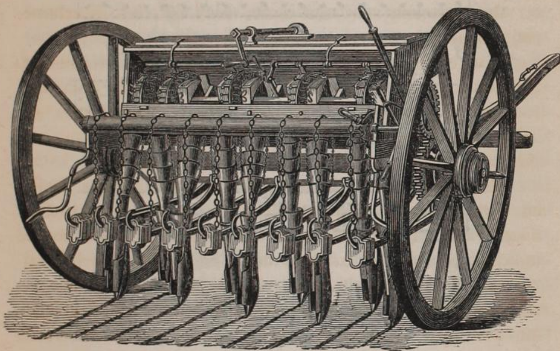
Fig. 8. Drillmaschine.
